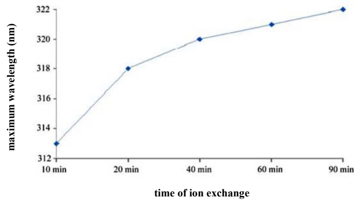
Figure 3: The wavelength of maximum absorbance of prepared samples.
