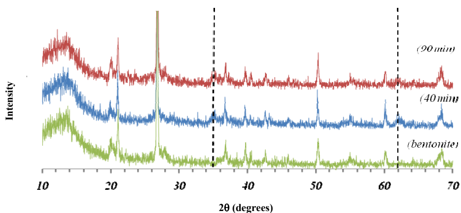
Figure 6: X-ray diffraction pattern of parent bentonite and Cu-MMT nanocomposites.
