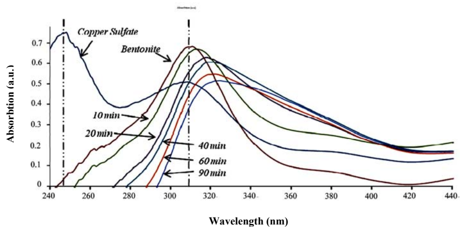
Figure 2: Diffusive reflectance spectra of prepared samples.
